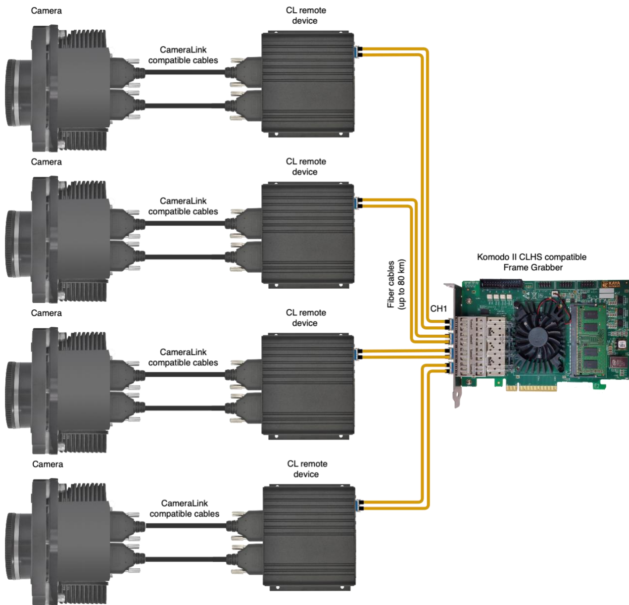
Figure 1 – KY-FXCL-II quad camera topology
