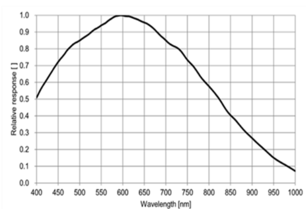
Mono Spectral Response Sony IMX 250
