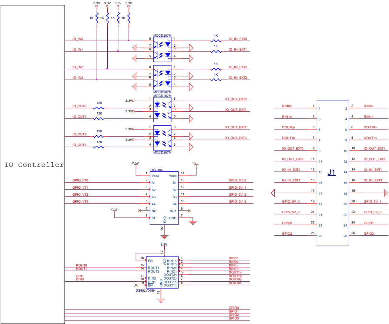
Figure 17 : GPIO Connector schematic
