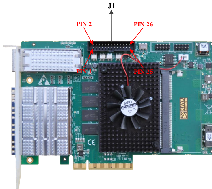
Figure 16 : GPIO connectors location
