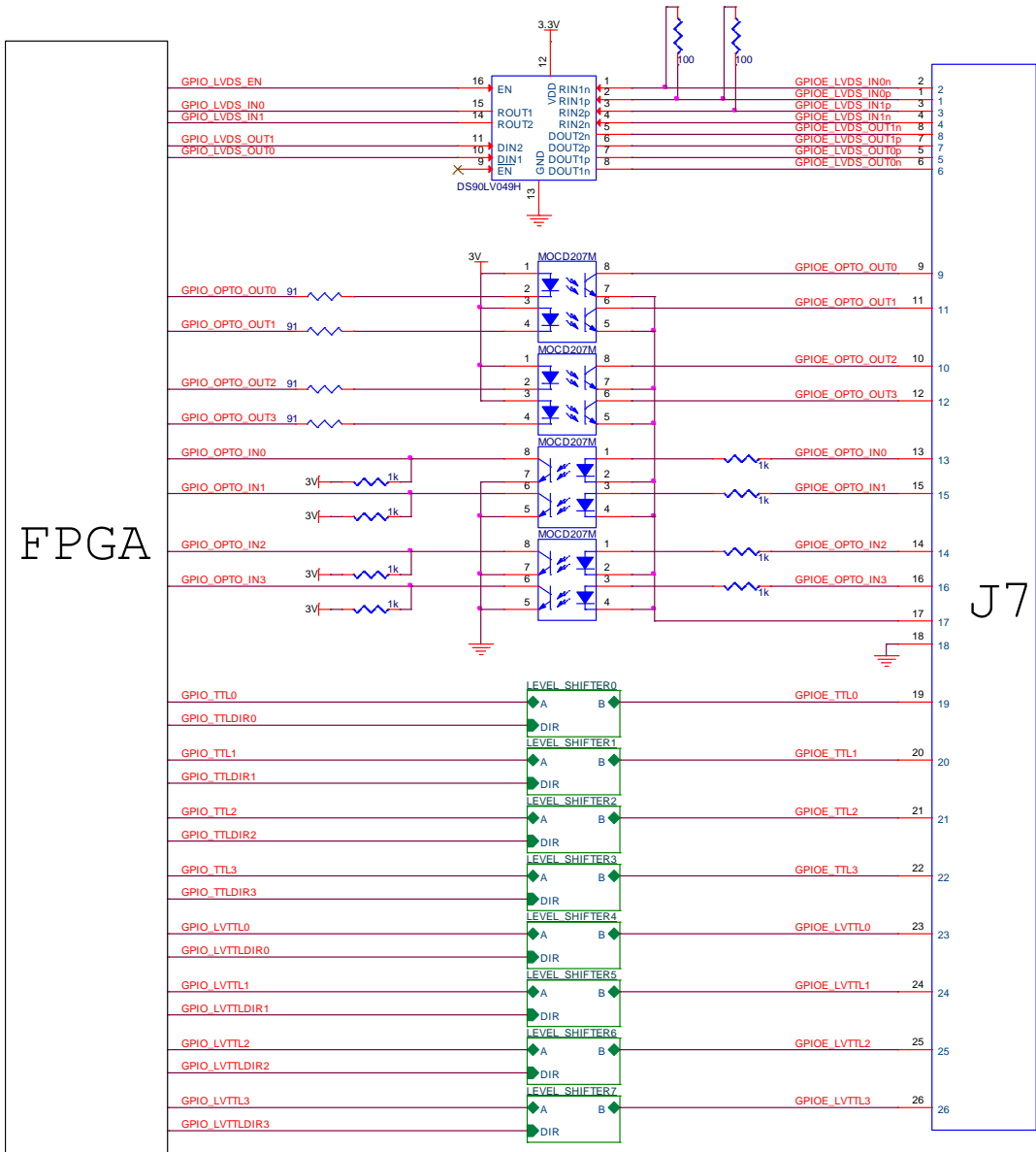
Figure 8: GPIO Connectors schematic
