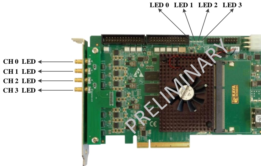
Figure 5: Komodo II Board LED’s locations
