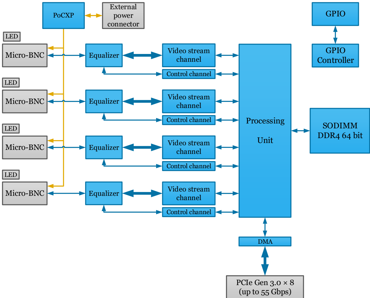
Figure 6: Komodo II Board Block Diagram
