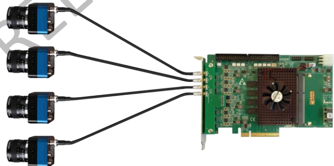
Figure 1: CoaXPress system block diagram
